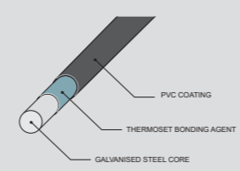
FUSE BONDED PVC WIRE
